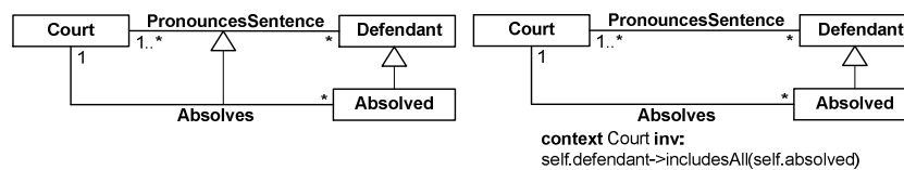
Fig.3.a-b Example of an association specialization and its translation
