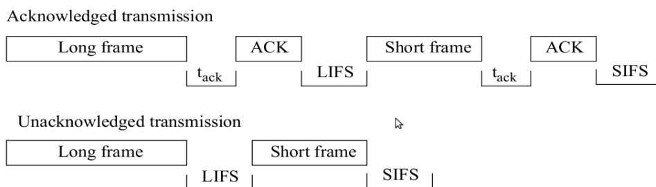
Figura 17 – IFS – Inter-Frame Space
